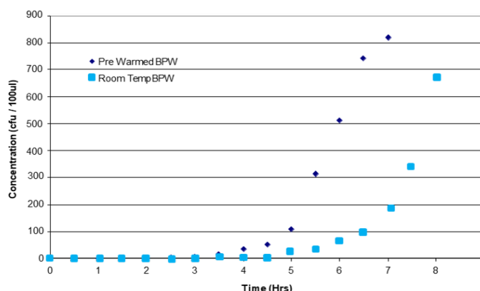
Figure 1. Salmonella growth in pre-warmed and room-temperature media
